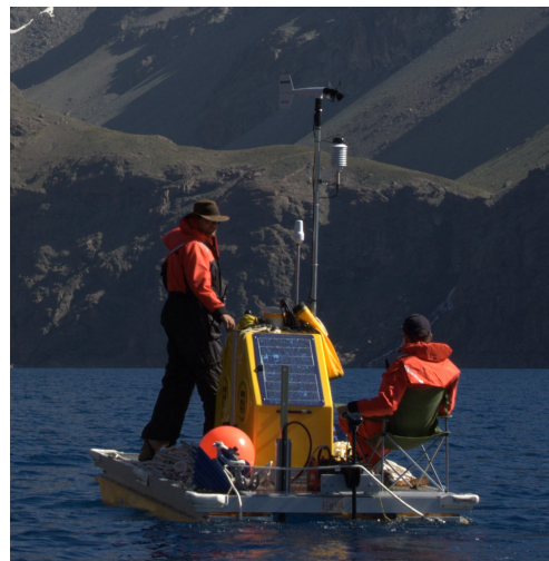
Figure 2: Deployment of Lake Lander 1.0 to Laguna Negra in December 2011
