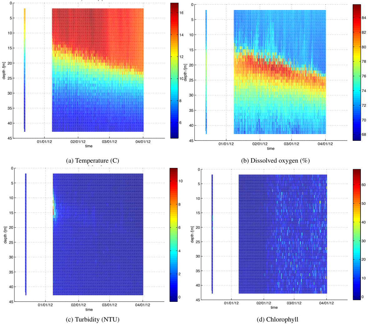
Figure 3: Lake Lander profiler data. Water quality parameters (temperature, turbidity, etc) from the surface to deep within the water column are plotted against time (December 2011 - April 2012). Summer warming of the lake is evident in the gradual lowering of the thermocline (a). It is hypothesized that photosynthetic organisms cluster around the thermocline as evidenced by the increased concentration of oxygen there (b), however there is no clear relation of the chlorophyll signature to depth (d). The tail end of a turbidity spike resulting from the discharge of summer time glacial meltwater is visible in (c).
