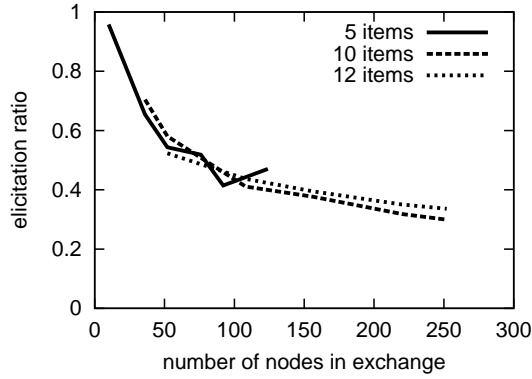
Figure 2: Scaling experiment: elicitation vs. exchange size.
